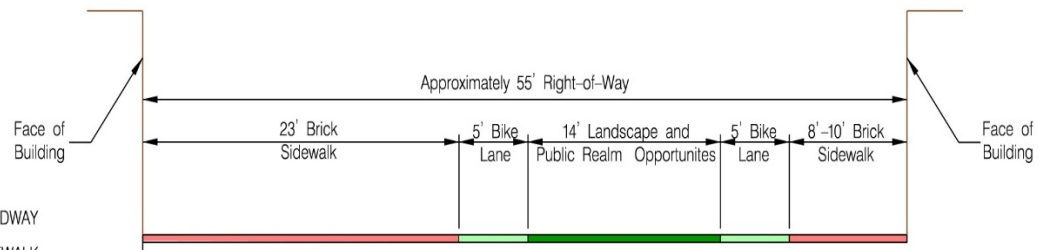
Baltimore Street Typical Section Looking from George St Towards Centre St
